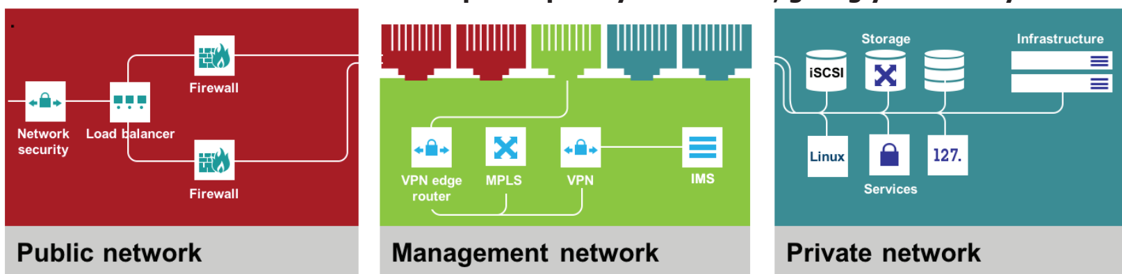
Figure 2 : Triple-network architecture
